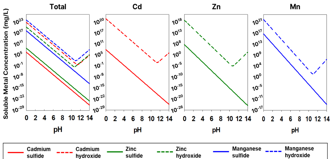
Fig. 1. Comparisons of solubilities for metal sulfides and metal hydroxides as a function of pH.
